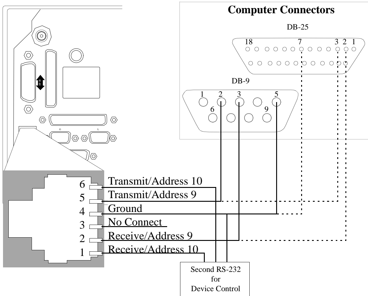
Figure 6 Connecting the HP 8924C/E Serial Port to a PC or Terminal
