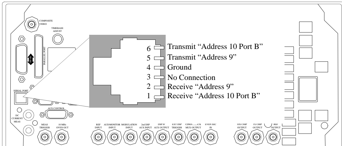
Figure 3 Serial Printer connection (HP 8924C/E)
