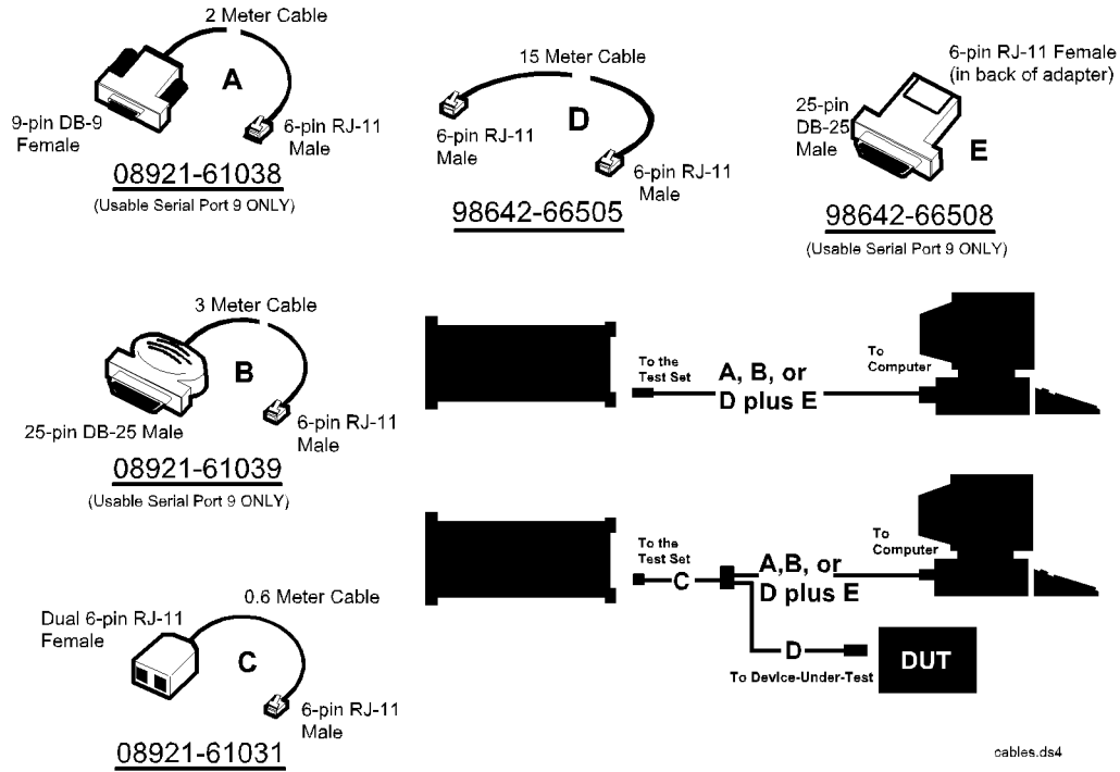
Figure 7 Available HP RS-232 Serial Cables and Adapters
